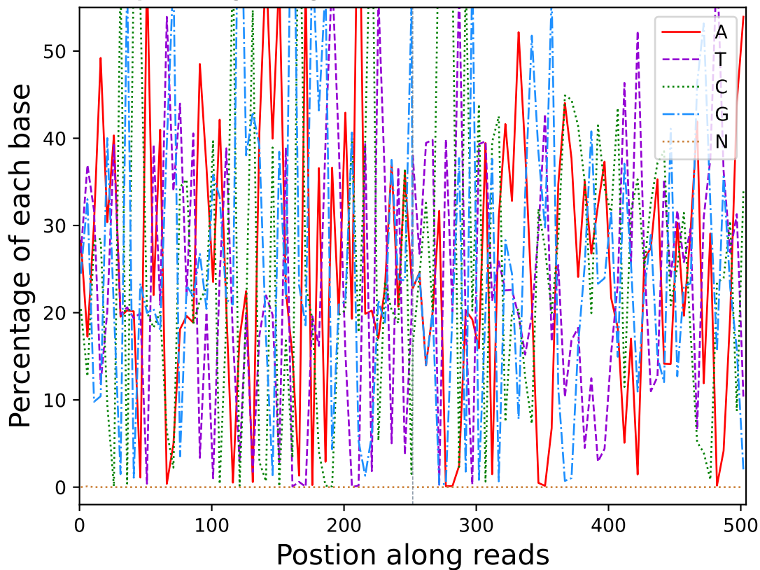
Base percentage along reads (R10319)
